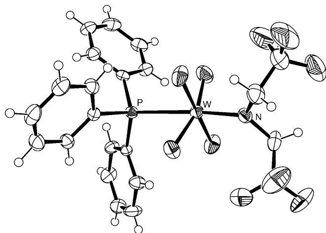
Figure 4. The structure of [(\text{CF}_3\text{CH}_2)_2\text{N}-\text{WF}_6-\text{P}(\text{C}_6\text{H}_5)_3] in the crystal, ORTEP representation, 50% probability ellipsoids.
